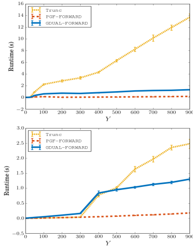
Figure 3. Running time vs. Y . Top: \rho = 0.15 , bottom: \rho = 0.85 .
