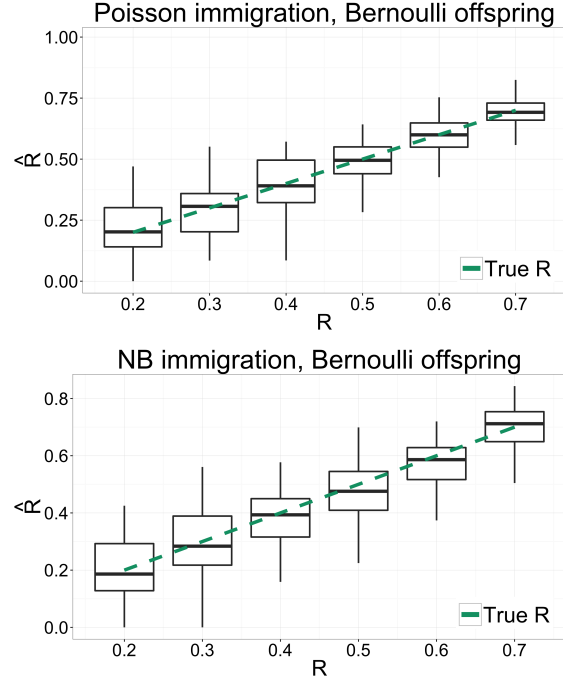
Figure 5. Estimates of R for two additional models. Titles indicate immigration and offspring distribution. 50 trials summarized as box plot for each model, parameter combination.
