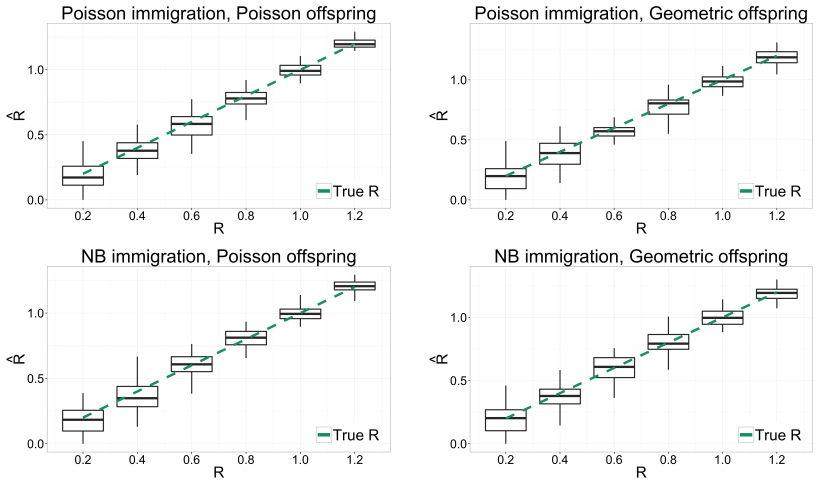
Figure 4. Estimates of R in different models. Titles indicate immigration and offspring distribution. 50 trials summarized as box plot for each model, parameter combination.
